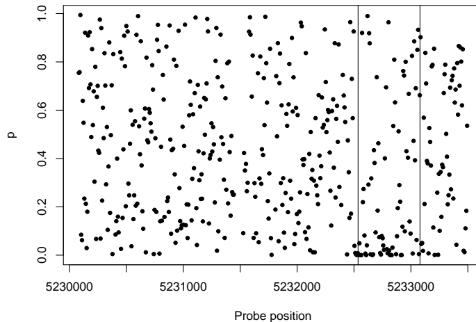
Figure 1: Probe-level p-values
