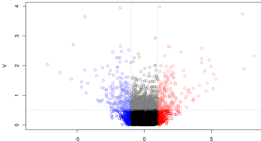
Figure 3: SV-plot produced from S_a GEVAQuantiles object using the geva.quantiles function using the initial.thresholds = c(S=1, V=0.5) parameter.
