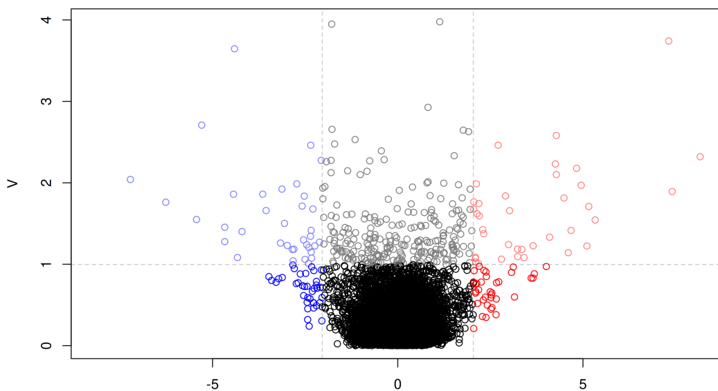
Figure 2: SV-plot produced from a GEVAQuantiles object using the geva.quantiles function with default parameters.
