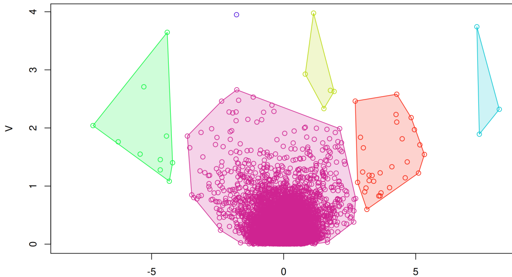
Figure 4: SV-plot produced from a S GEVACluster object using the geva.cluster function with the hierarchical method and 30% of resolution.
