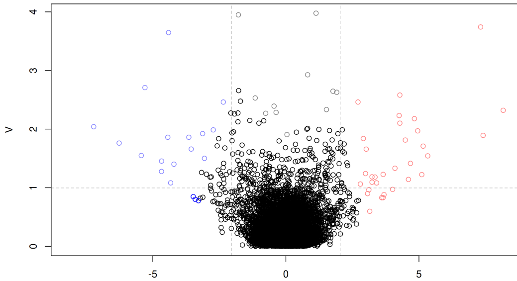
Figure 6: SV-plot produced from a S GEVAResults object using the geva.finalize function with 0.05 as p-value cutoff.
